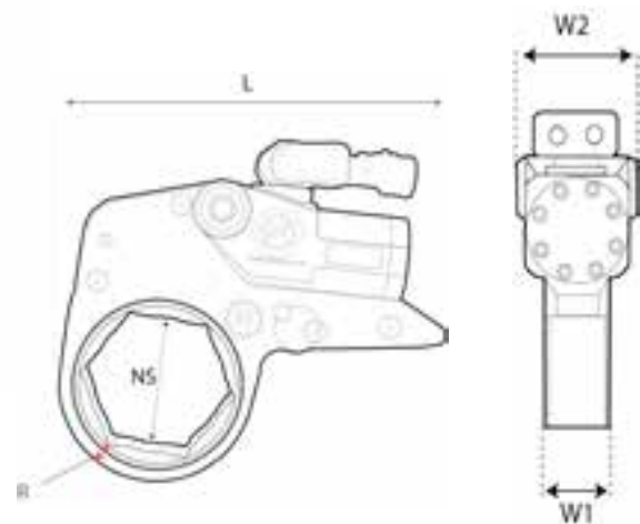
RTX Direct fit low profile dimensions
