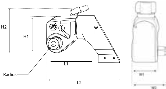
Square Drive hydraulic torque wrench dimensions
